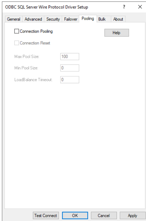
Figure 5: Pooling tab
