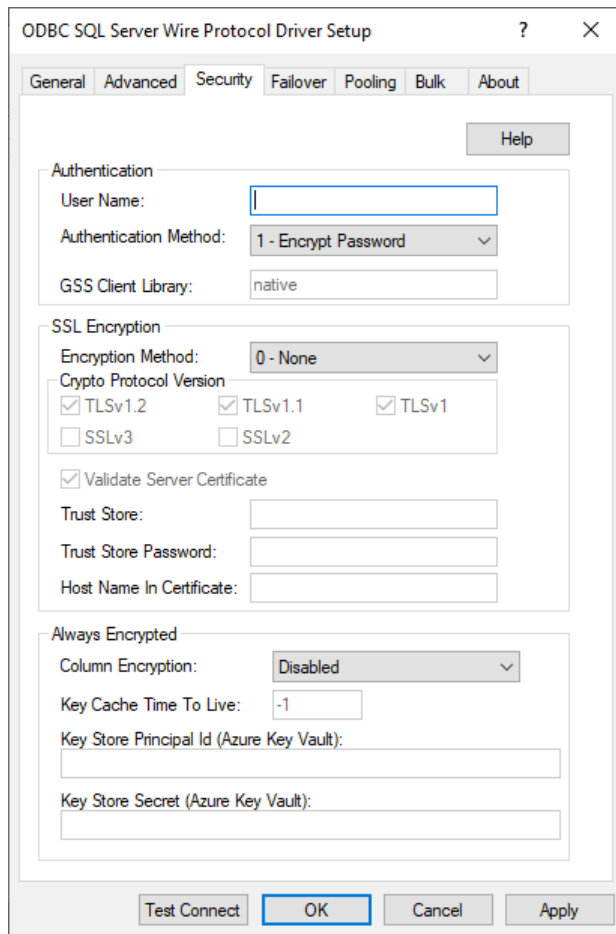
Figure 3: Security tab
