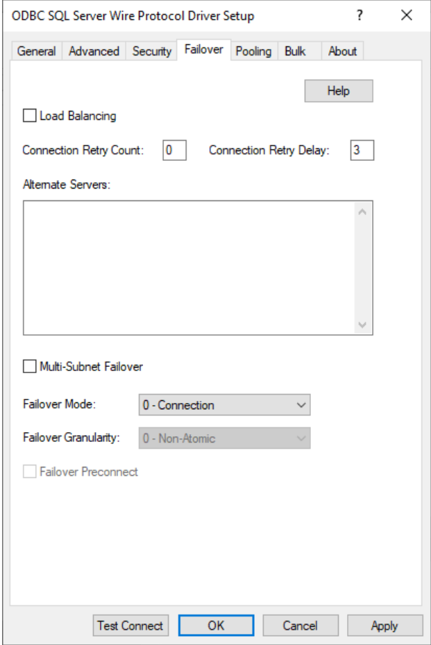
Figure 4: Failover tab
