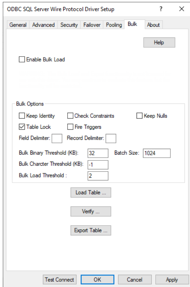
Figure 6: Bulk tab
