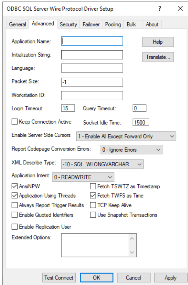
Figure 2: Advanced tab
